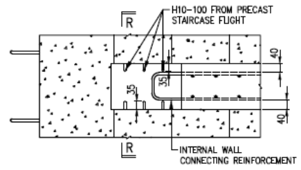
DETAIL 'F': STAIRCASE FLIGHT REINFORCEMENT CAST IN-SITU LOCATION
