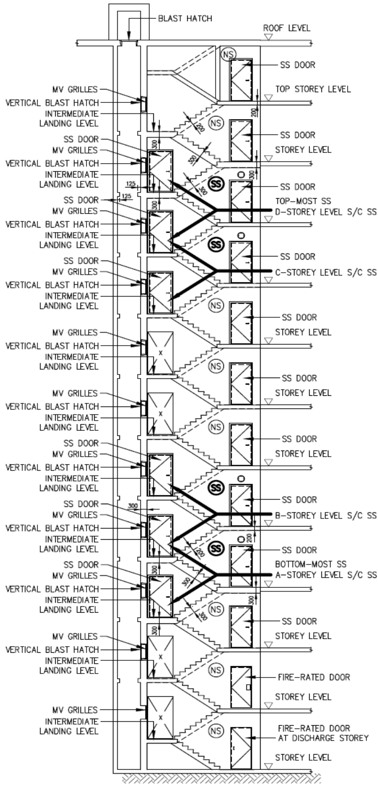
FIGURE 2.12.1(a): SECTION X-X OF S/C SS WITH SS/NS
