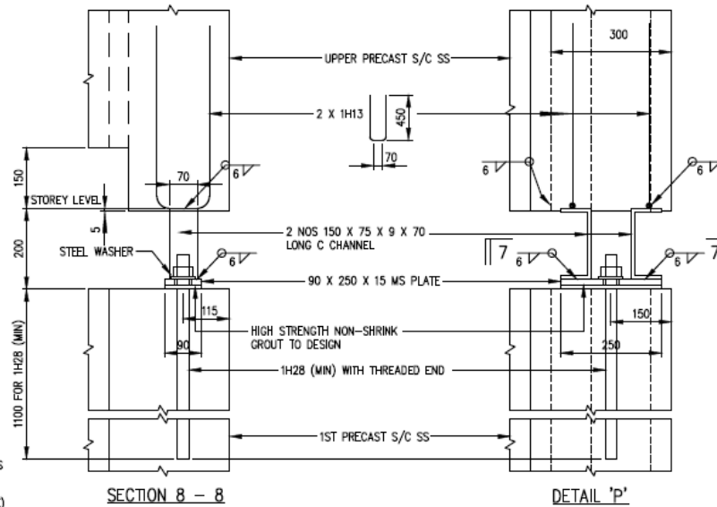
SECTION 8 - 8
