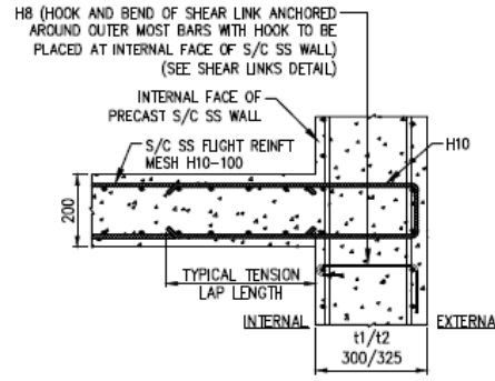
SECTION N-N: SECTION OF STAIRCASE FLIGHT AT RIB
