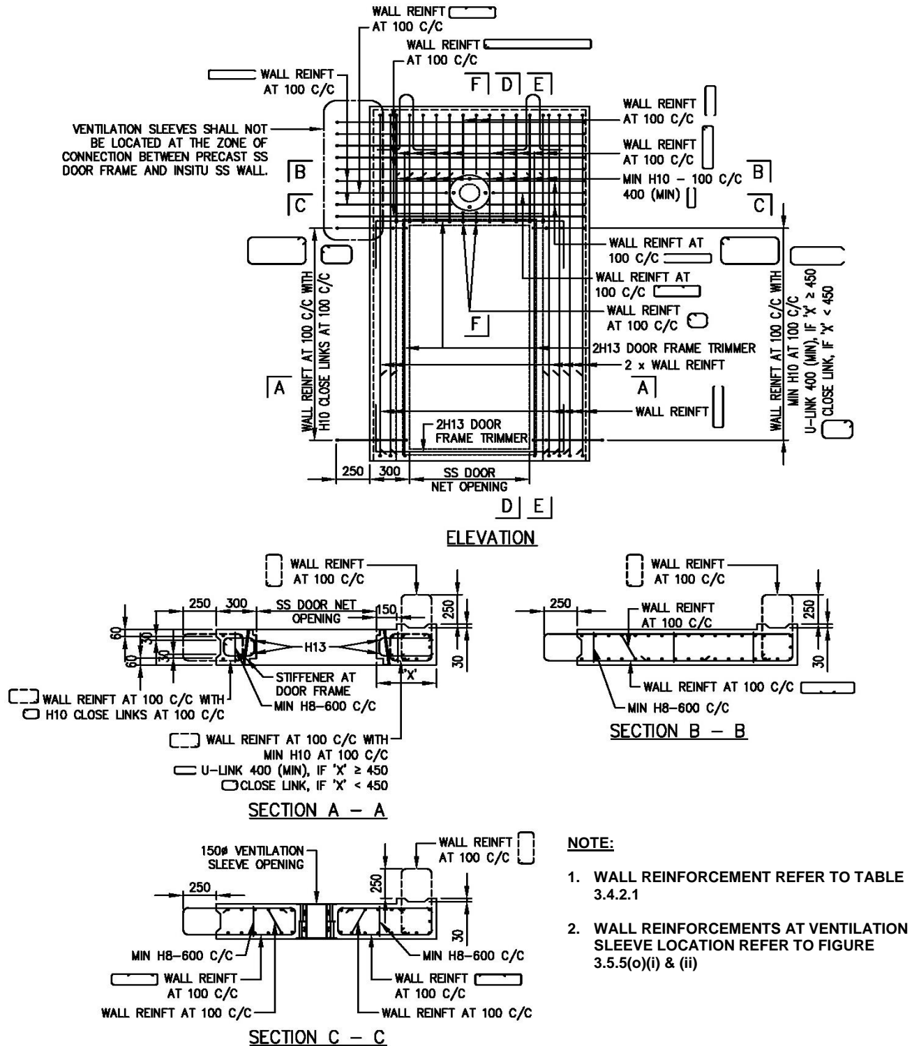
FIGURE 3.5.5(g): DETAILS AND SECTIONS OF PRECAST SS DOOR FRAME PANEL WITH VENTILATION SLEEVE ABOVE IT (TYPE 2)
