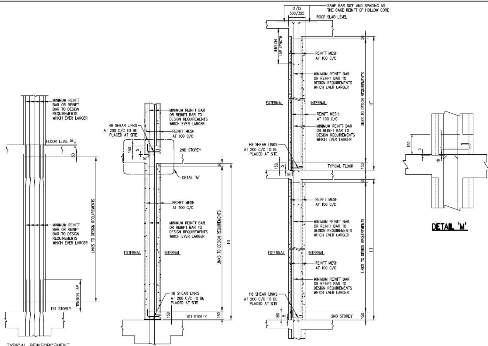
FIGURE 3.5.6.2(k): REINFORCEMENTS LAPPING IN HOLLOW CORES
