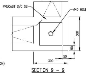
SECTION 9 - 9
