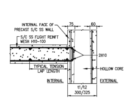
SECTION M-M: SECTION OF STAIRCASE FLIGHT AT HOLLOW CORE
