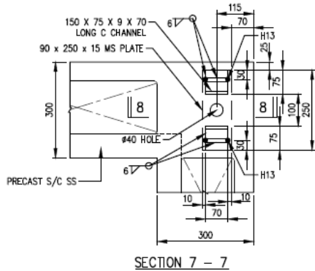
SECTION 7 - 7
